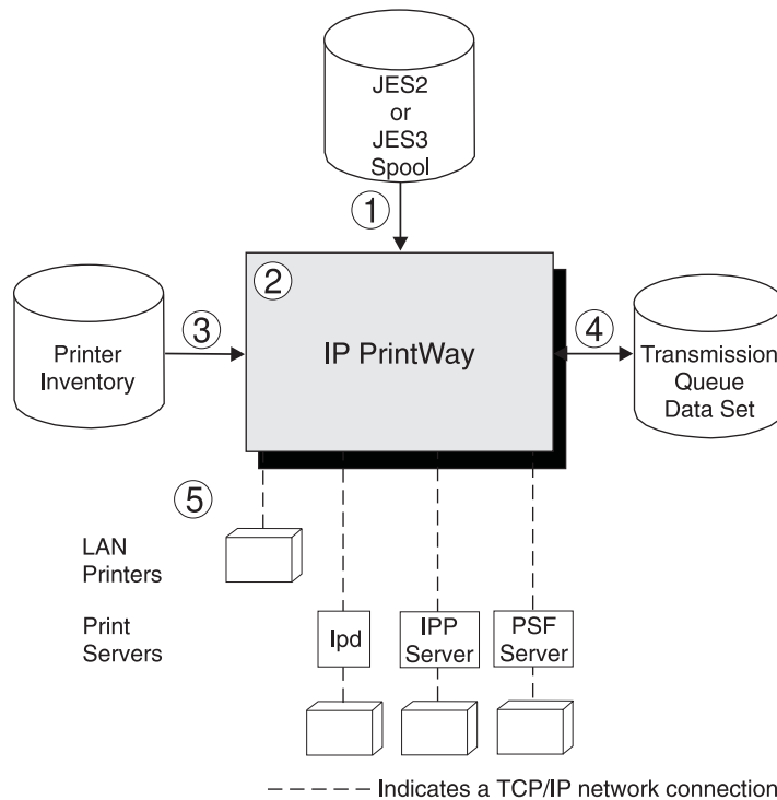
Figure 8. IP PrintWay System Diagram
